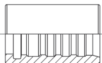
PF-7 Smooth Bore PTFE SAE 100 R14
